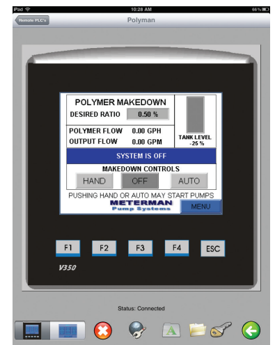
Sample Screenshot
